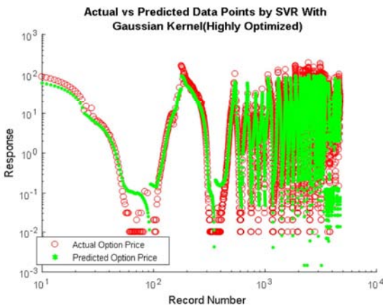
Figure 10. Logarithmic Response Plot of Gaussian SVR (Highly Optimized).
