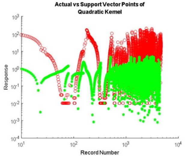
Figure 12. Logarithmic Support vector of SVR with Quadratic Kernel.
